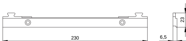
Lateral spacer for striking plates cod.
